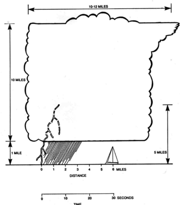
Figure 1. Thunderstorm ranging using time to thunder.
