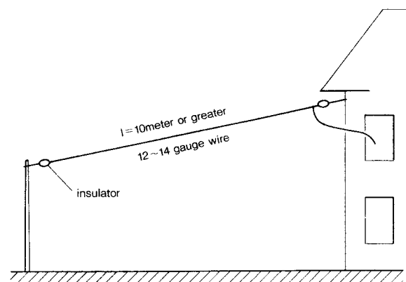
Long-Wire Antenna Construction
