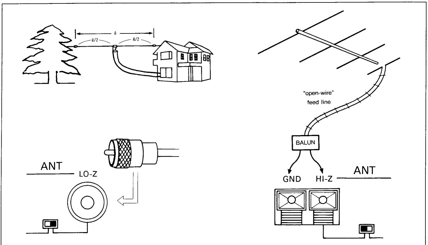
Typical HF Antenna Installation
