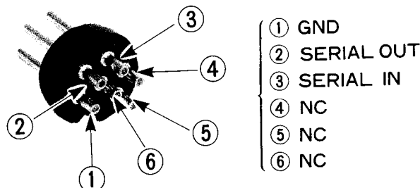
CAT System Jack Pin-Out Diagram
