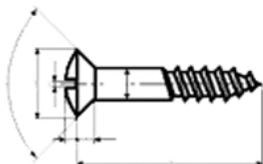
vis-bois-TFB-fendue-R95.gif
