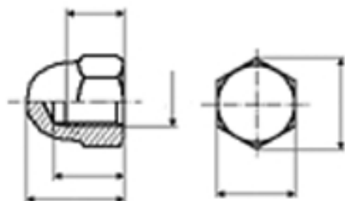
ecrou-borgne-R1721.gif
